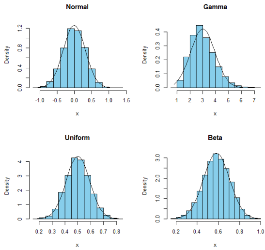
sample size = 50
