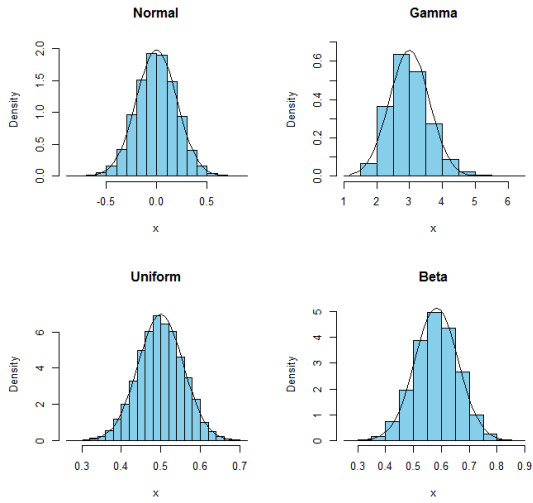
sample size = 100
