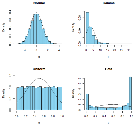
sample size = 1
