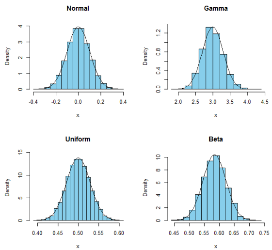
sample size = 100
