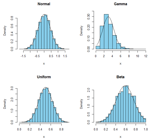
sample size = 5
